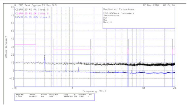
Figure 8-34. Radiated EMI Rod Antenna
